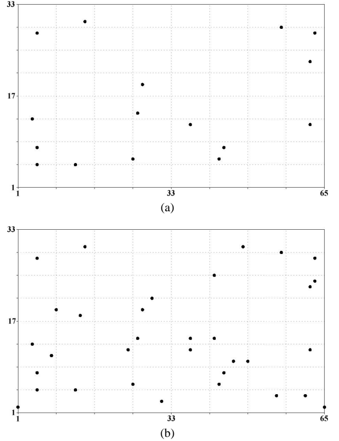
Fig. 2. Horizontal distribution of the rawinsonde locations for (a) the 16 stations experiments and (b) the 32 stations experiments.
