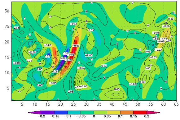
Fig. 8. Same as Figs. 6a or 6b but with the bred vector obtained using a streamfunction norm. Note that in Fig. 6 the bred vectors were obtained using potential vorticity norm.
