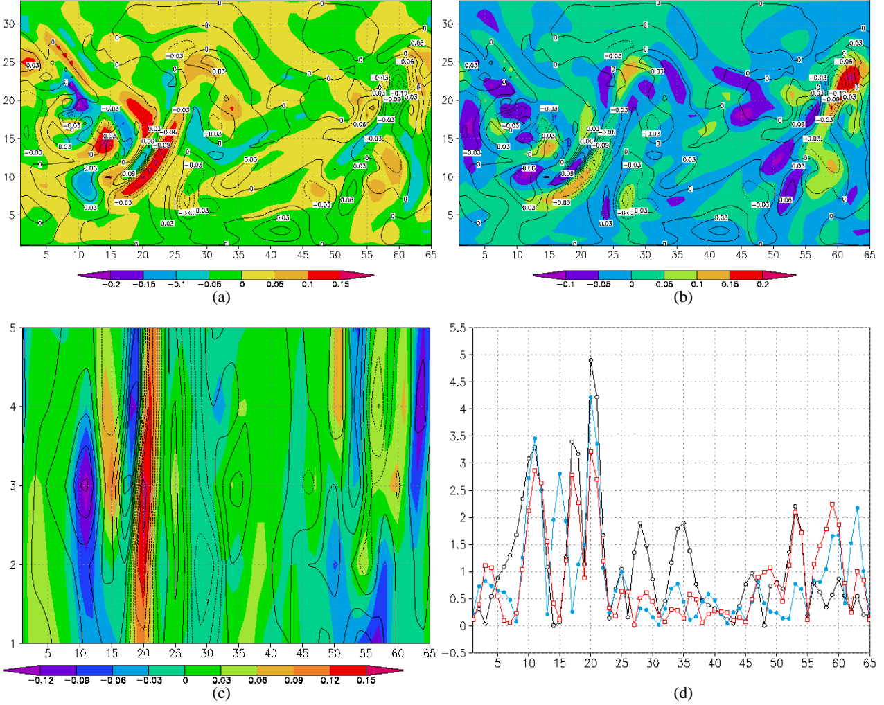
Fig. 6. (a) and (b) Two randomly chosen bred vectors for a medium density observing network (32 rawinsondes) (color shaded). Contours represent the corresponding background error. (c) vertical cross-section of the same vectors in (a) ( y = 10 ). (d) same as Fig. 4d for the vectors represented in Figs. 6a and 6b [ y = 10 ].
