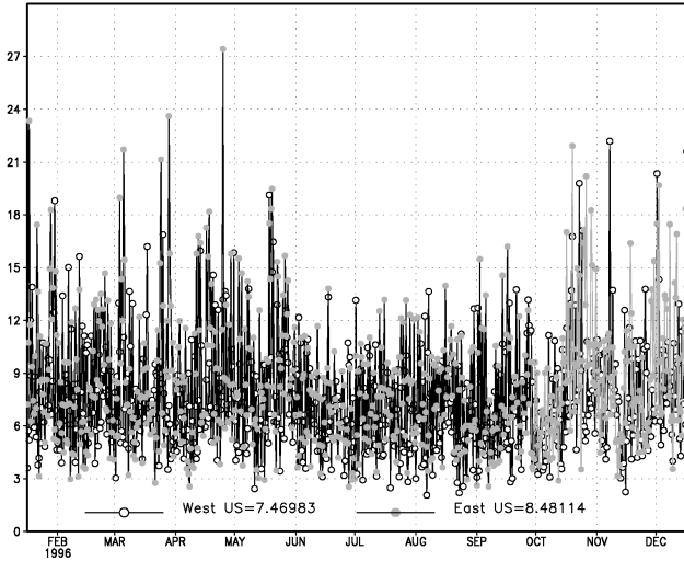
Fig. 1. Root mean square analysis increment in the 500 mb geopotential height for the NCEP 50 year reanalysis during 1996 over the western (open circles) and eastern (gray dots) portions of the US.
