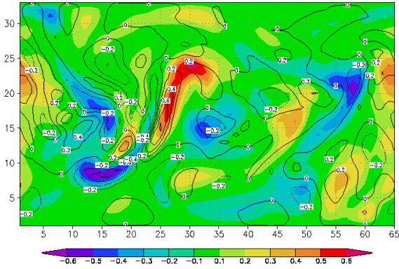
Fig. 5. Background error (contour) and a bred vector (color shaded) obtained with a breeding cycle based on the truth. The figure should be compared with Figs. 4a and 4b where the breeding cycle is based on the analysis.
