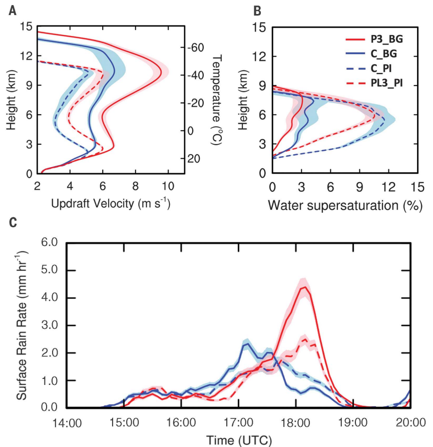
Fig. 3. Simulated aerosol effects on the DCCs.
