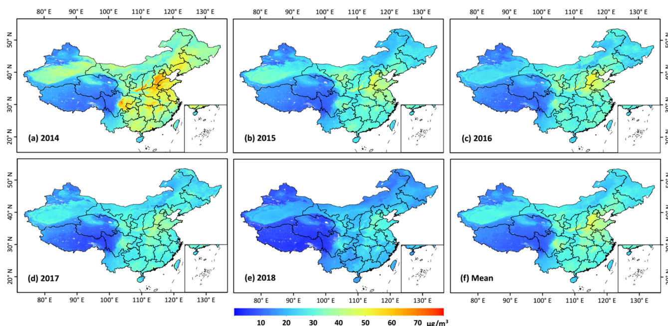
Figure 3. Satellite-derived 1-km-resolution annual mean \text{PM}_{10} concentrations across China from (a)–(e) 2014 to 2018 and (f) for all years.
