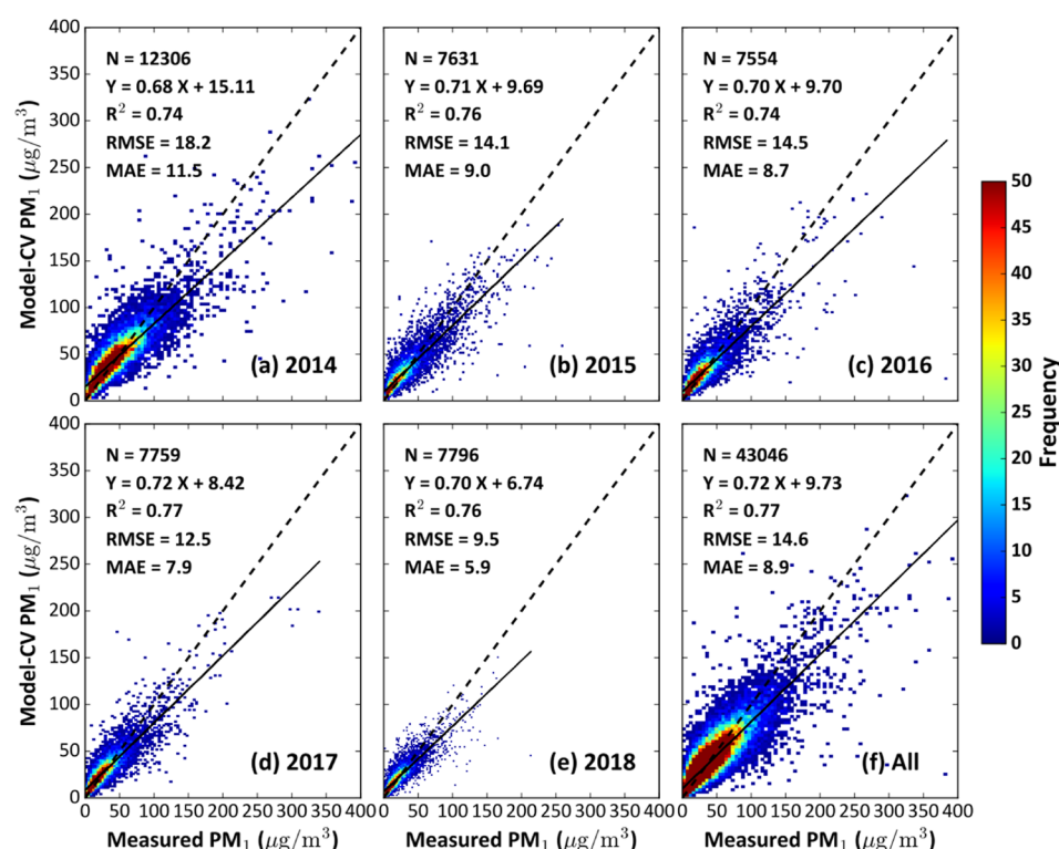
Figure 1. Density scatterplots of 10-fold cross-validation results of 1 km daily PM 1 estimates across China for the years (a)–(e) 2014 to 2018 and (f) all years. Statistical metrics are given in each panel: the number of samples ( N ), the coefficient of determination ( R 2 ), the root-mean-square error (RMSE), and the mean absolute error (MAE). The linear regression relationship is also given in each panel. Dashed lines are the 1:1 lines, and solid lines are the linear best-fit lines through the data points.
