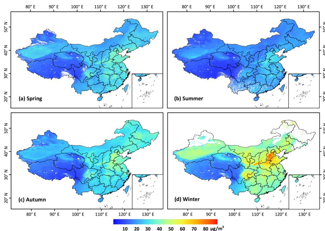
Figure 4. Seasonal mean 1-km-resolution \text{PM}_{10} concentrations in (a) spring, (b) summer, (c) autumn, and (d) winter during 2014–2018 across China, respectively.
