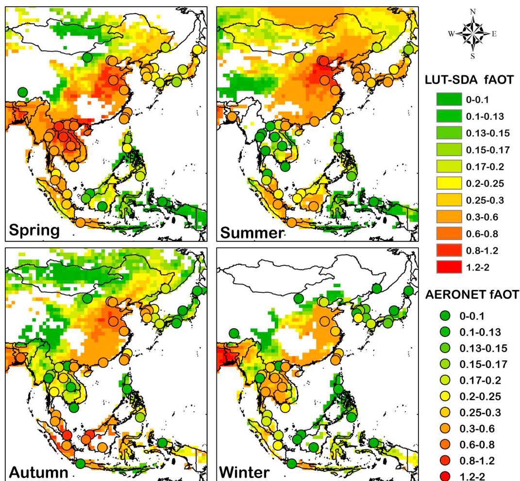
Fig. 7. Seasonal mean faOT from the LUT-SDA (background colors) and from AERONET (colored filled circles). (For interpretation of the references to color in this figure legend, the reader is referred to the web version of this article.)
