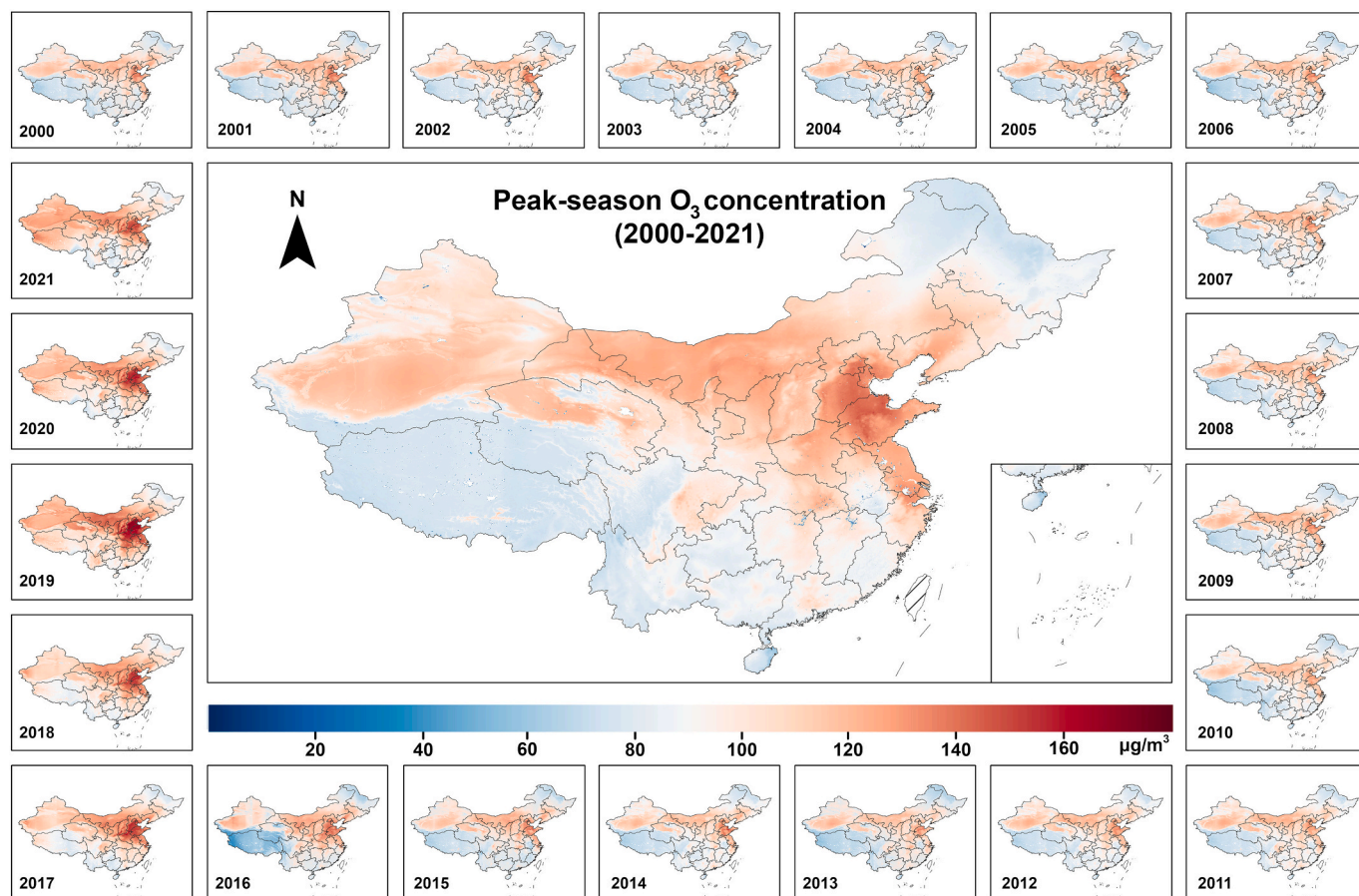
Fig. 4. Average peak-season surface O_3 maps at a 1-km resolution spanning 2000 to 2021 for mainland China. The central map shows the 22-year average, and smaller maps surrounding it show maps for each individual year.
